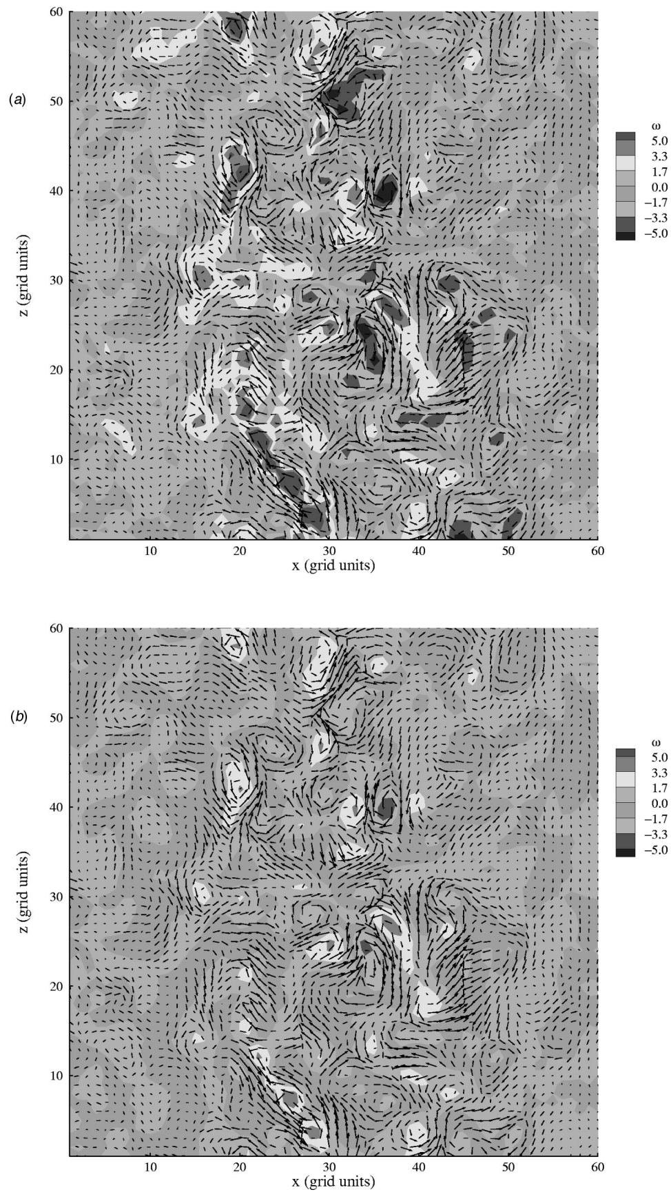
Fig. 5 Vorticity obtained by differentiating (a) instantaneous and (b) high-pass filtered field with overlaid high-pass field vectors
