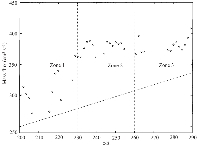
FIGURE 14. Variation of mass flux for \diamond , a heated jet. —, normal jet ( Re=2400 , G=4.3 ). Note that the mass flux in zones 2 and 3 is an under estimate of the true mass flux (see the accompanying text).
