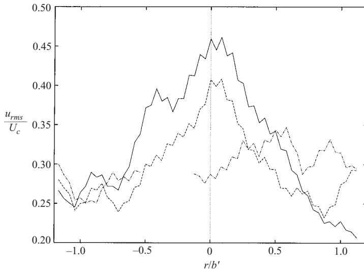
FIGURE 10. Normalized fluctuations of the streamwise velocity in the three zones. Key as in figure 6. Re = 2400 , G = 4.3 , b' is the nominal jet width corresponding to the mid- z location of the viewframe. (Zone 3 data for -0.5 < r/b' < -0.2 was corrupted by strong localized reflections from the wire grids and are omitted).
