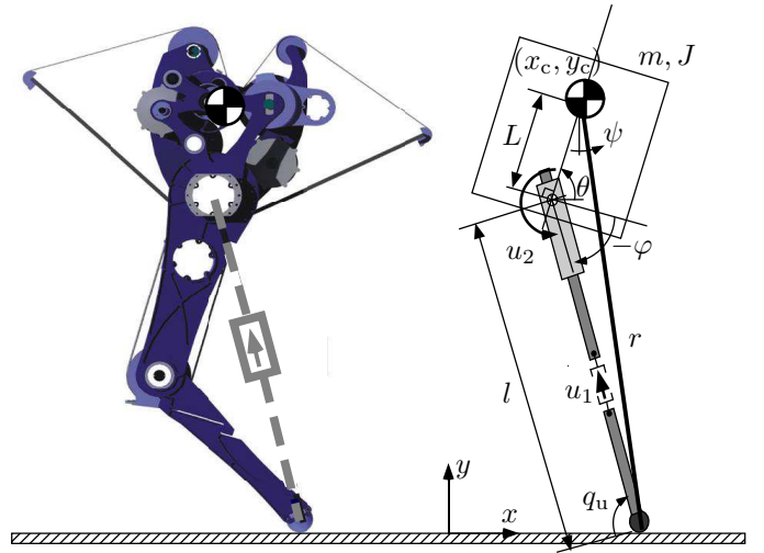
Fig. 1. Left: A mechanical drawing of the monopedal robot Thumper constructed in a collaborative effort between the University of Michigan and Carnegie Mellon University; see [22], [23], and [24] for design principles. The knee has a revolute series compliant actuator. Right: The Asymmetric Spring Loaded Inverted Pendulum (ASLIP). The leg force u_1 will be modeled as a spring in parallel with a prismatic force source. The ASLIP is a more faithful representation of the robot on the left than a SLIP model.
