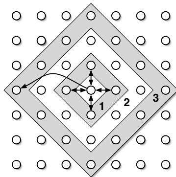
Fig. 2. A small-world graph, after Kleinberg Kleinberg (1999). The nodes inside the shaded diamonds have the same Manhattan distance to the node in the center. This simple lattice network is conceptually related to the small-world model of Watts and Strogatz (1998). Nodes in area 1 are bi-directionally connected to the center node, which is also uni-directionally connected to one node in area 3.
